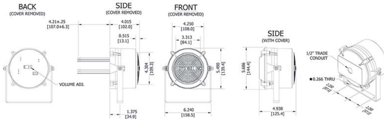
DIMENSIONS ARE IN INCHES [ mm ], TOLERANCES ARE ±0.03in [±0.76mm] UNLESS OTHERWISE SPECIFIED.
