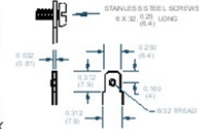
"S" TERMINALS
