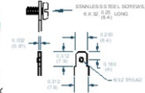
"S" TERMINALS
